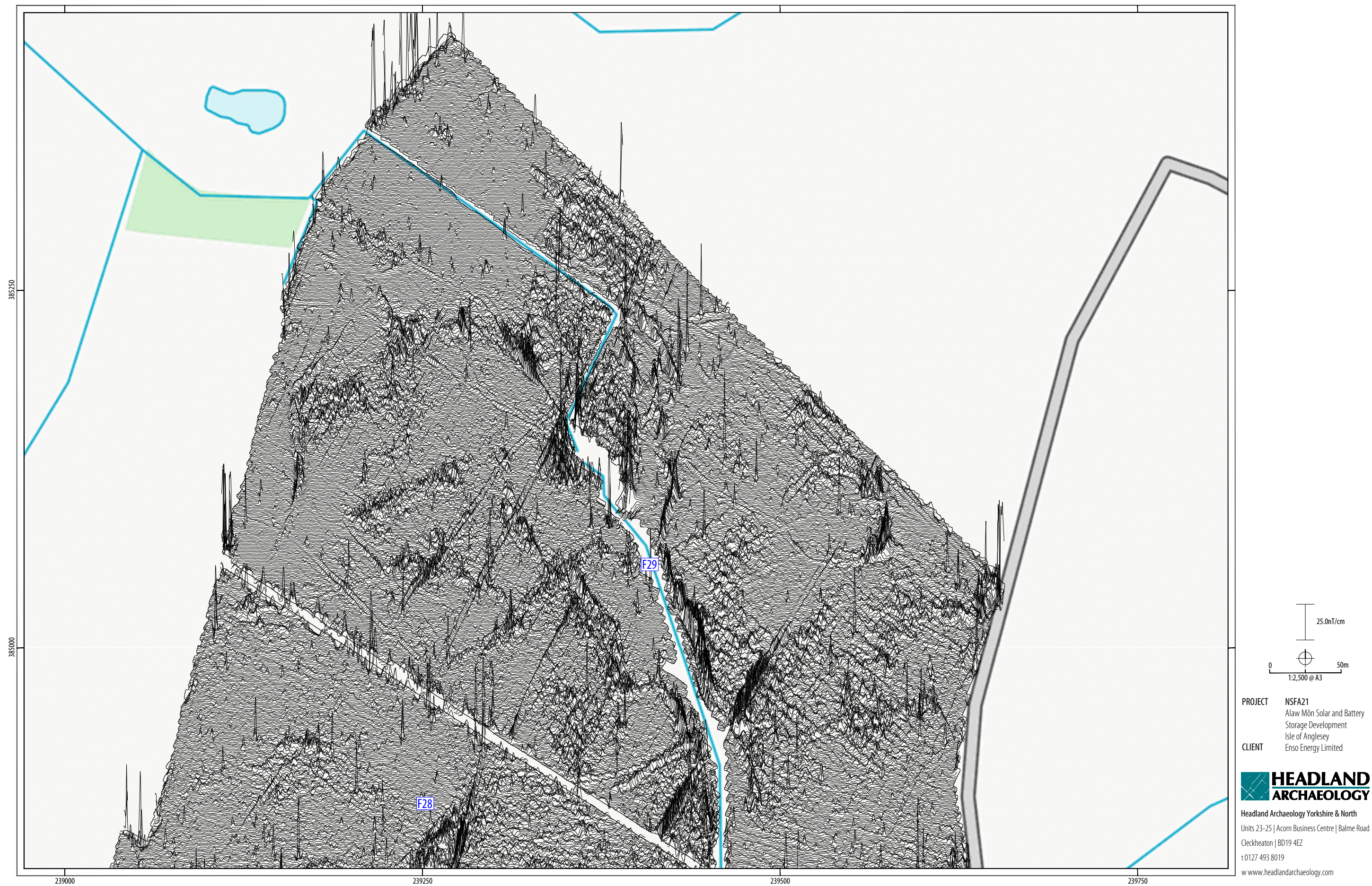
ILLUS 28 XY trace plot of minimally processed magnetometer data; Sector 6
